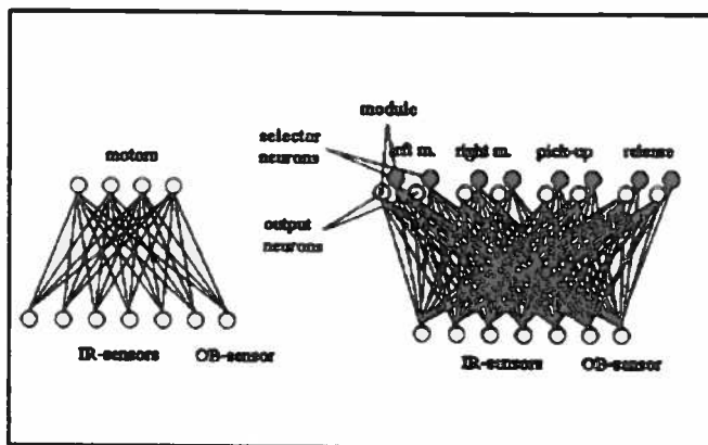
Figure 2 Architectures (a) and (b) are shown on the left and right side, respectively. Architecture (a) is used in the nonmodular population. Architecture (b) is used in the two modular populations (i.e., in both hardwired and duplication-based modular populations). However, in the hardwired modular population two modules compete to gain control of each of the four actuators. In the duplication-based modular population individuals of the initial generation have only one module for each motor, that is, they initially have architecture (a). A second competing module may be added in individuals of successive generations as a result of the duplication operator. Another difference is that in the hardwired modular population competing modules have different random weights from the beginning, while in the duplication-based modular population, when a second competing module is introduced, the two competing modules have identical weights.
